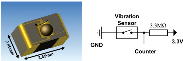
Fig. 2. The Micro Vibration Sensor from [2] and Schematic
